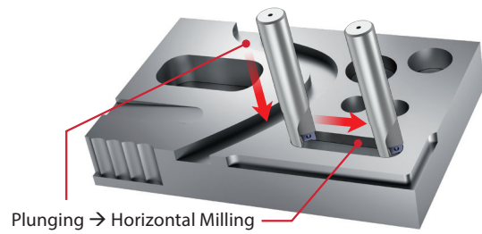
Plunging → Horizontal Milling
